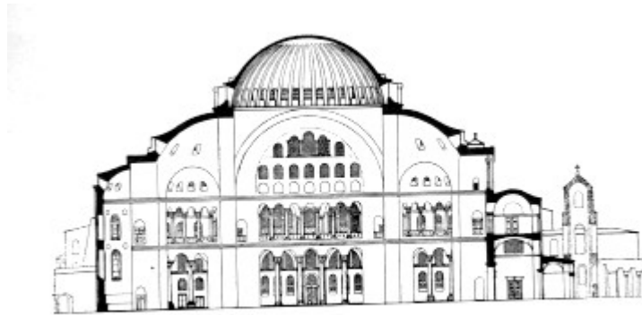
66 Sancta Sophia, Istanbul. Section after A. M. Schneider
